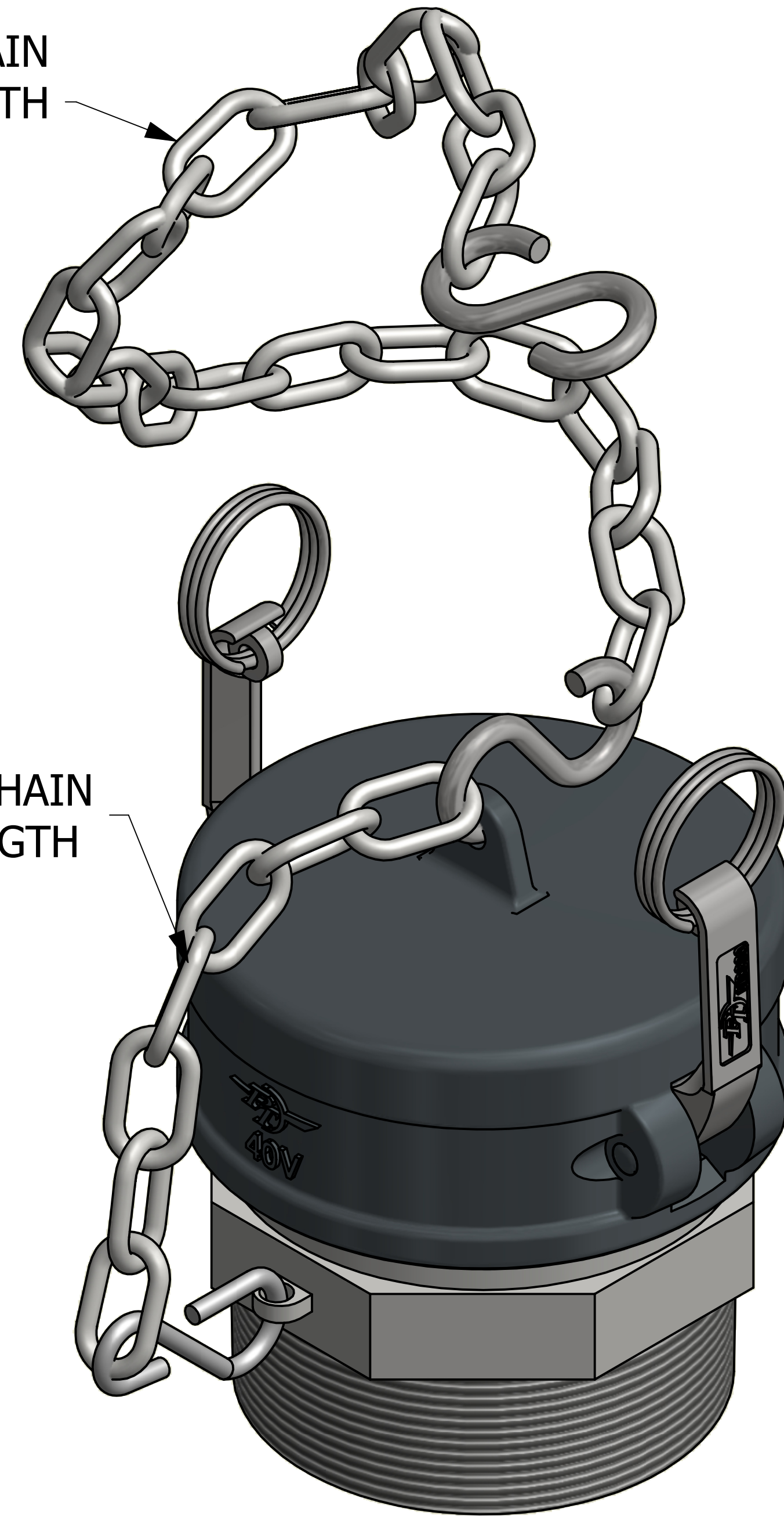
ISOMETRIC VIEW
